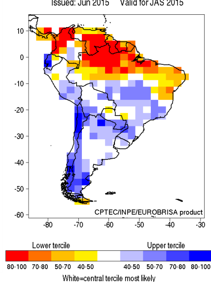
Integrated: Prob. of most likely precip. tercile (%) Issued: Jun 2015 Valid for JAS 2015
