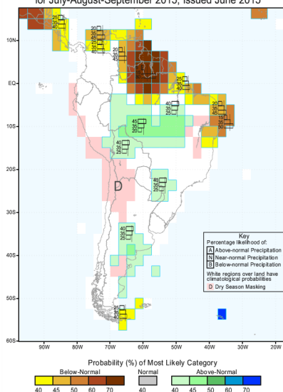
IRI Multi-Model Probability Forecast for Precipitation for July-August-September 2015, Issued June 2015
