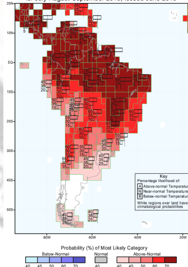
IRI Multi-Model Probability Forecast for Temperature for July-August-September 2015, Issued June 2015
