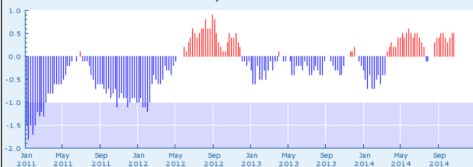
Weekly NINO3.4 index
