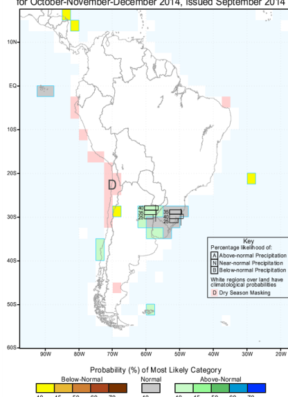
IRI Multi-Model Probability Forecast for Precipitation for October-November-December 2014, Issued September 2014
