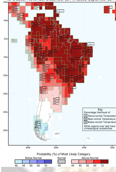
IRI Multi-Model Probability Forecast for Temperature for October-November-December 2014, Issued September 2014
