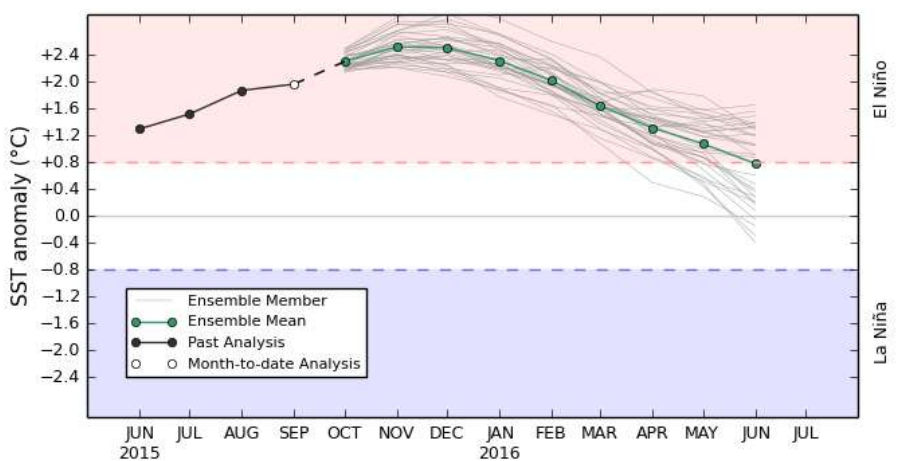
POAMA monthly mean NINO34 - Forecast Start: 27 SEP 2015
