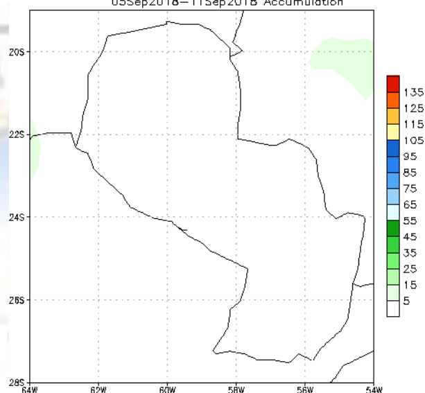
NCEP GFS Ensemble Forecast 1-7 Day Precipitation (mm) from: 05Sep2018 05Sep2018-11Sep2018 Accumulation
